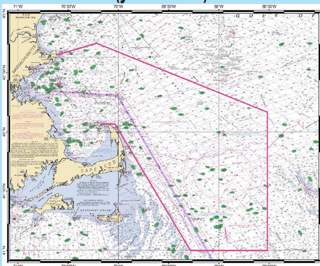
NOAA Chart #13009
